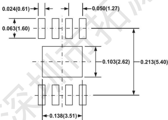
Land Pattern
